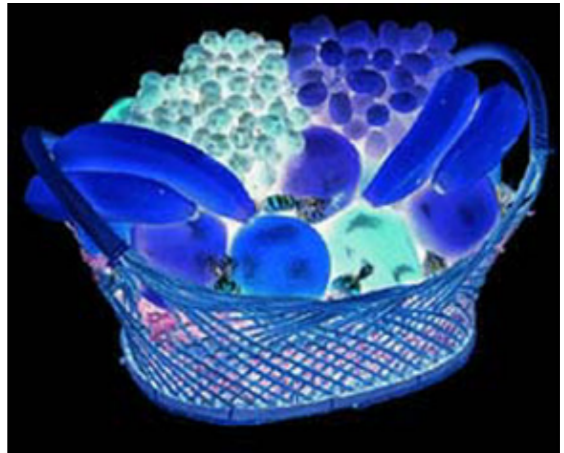
Inversion
